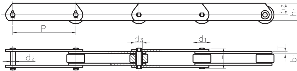
FVT SERIES CONVEYOR CHAINS
